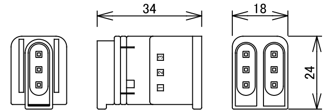
CTK3 (3 pin)
