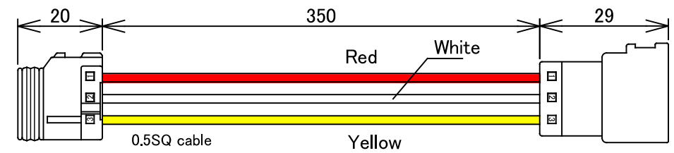
WCSHL-3TC (3 pin)
