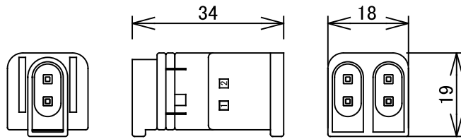
CTK2 (2 pin)
