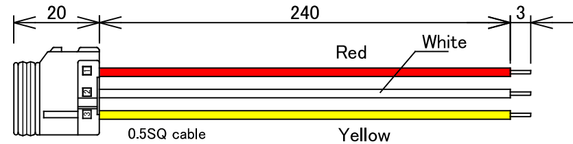
WCSHL-3PC (3 pin)
