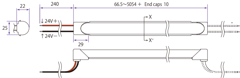
X-X' Cross section
