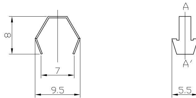
The sectional view of A-A'
